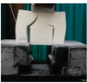
Compact Shear
