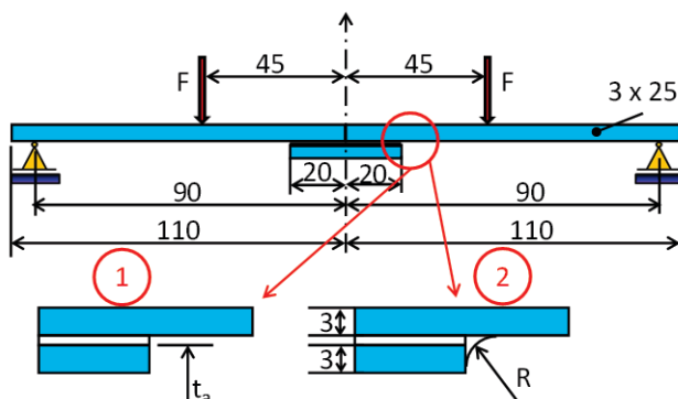
Geometry of the adhesive joint under four point bending
