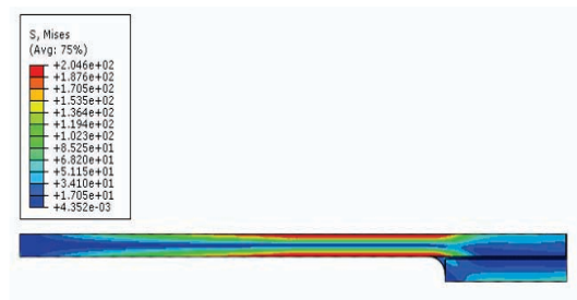
Equivalent stress distribution for the adhesive joint under four point bending
